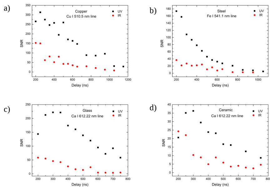
Fig. 1 Comparison of UV and IR LIBS signal to noise ratios of Cu I 510.5 nm spectral line on copper (a), Fe I 541.1 nm line on steel (b), Ca I 612.22 nm line on glass (c) and ceramic (d).
