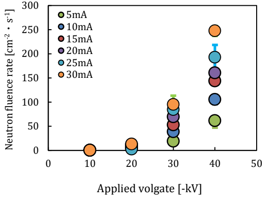
Figure 2: Dependence of neutron fluence rate on applied voltage
