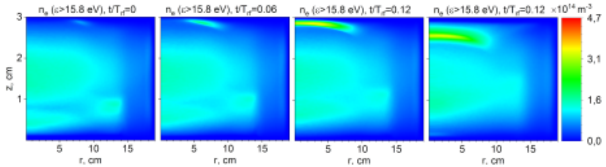
Fig.4: Evolution of an energetic electron population at the grounded electrode as a result of the excitation of surface wave at r = 8 cm, shortly before t=0 .
