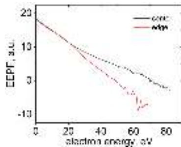
Fig.3: Electron energy probability function obtained from the described simulation, sampled at the discharge center (black) and the edge of the powered electrode (red).
