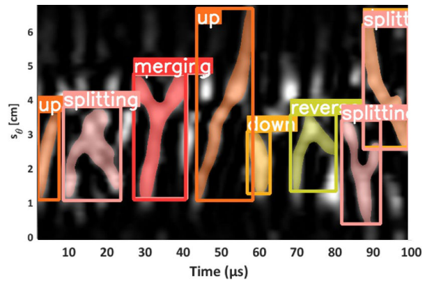
Figure 1: Light kymograph along the separatrix after tomographic inversion, showing various kinds of filament interactions detected using machine learning technique.
