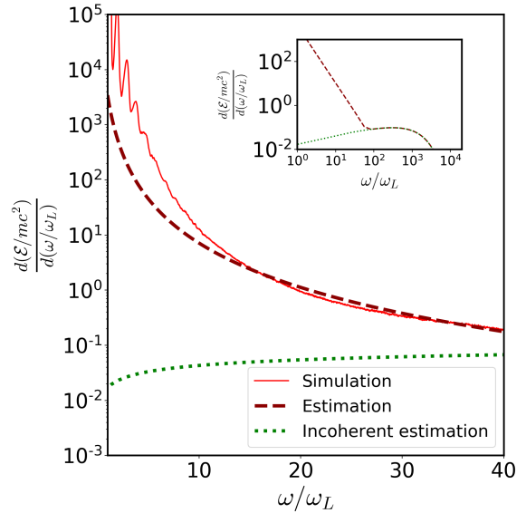
Figure 1: Radiation spectrum of the cold bunch of electrons (density n = 10^{20} \text{ cm}^{-3} , volume V = 0.125 \mu\text{m}^3 ) colliding with an intense ( I = 2.7 \cdot 10^{20} \text{ W/cm}^2 ) laser pulse. Red solid line – 3D PIC simulations result, dark red dashed line – estimation based on the developed analytical theory, green dotted line – incoherent radiation of N = nV electrons in the bunch. Inset: coherent and incoherent estimations of the spectrum in a wider frequency range.
