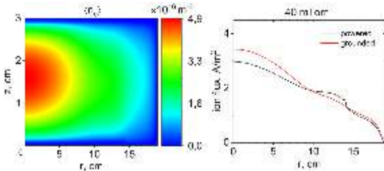
Fig.1: Time-averaged electron density and ion flux radial profiles at the powered and grounded electrodes obtained from a simulation of a CCP discharge in argon at 40 mTorr, driven at 106 MHz and 37 W.
