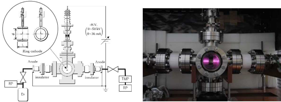
Figure 1: Schematic drawing and photograph of a compact neutron source by a high voltage ring-shaped cathode discharge.
