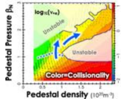
Fig. 1: High shaping accesses high pressure & density at low v^*
