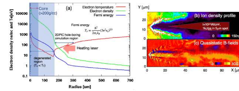
Fig. 1: (a) Density and temperature profiles of the imploded solid ball obtained by a hydrodynamics code, PINOCO. (b) A kJ petawatt laser light is capable of hole-boring in a coronal plasma beyond 100s of the critical density, simulated by a particle-in-cell code, PICLS.
