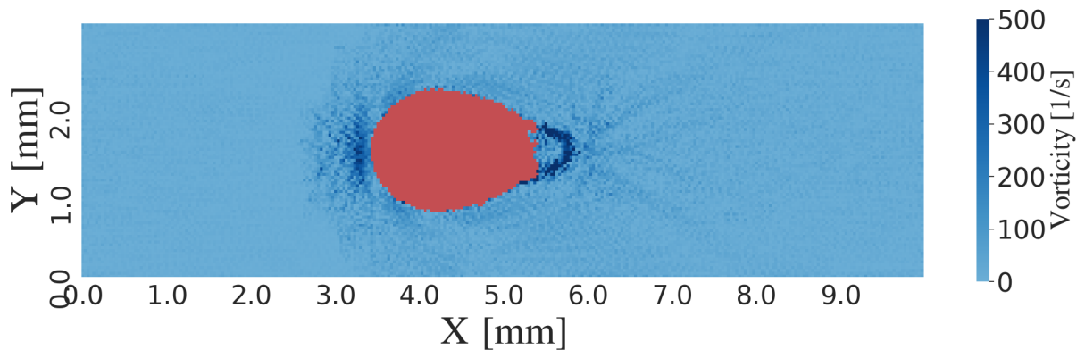
Figure 1: Vortices around an obstacle due to supersonic flow. The vorticity is averaged over one second in bins of size 0.03 \times 0.03 \times 0.2 \text{ mm}^3 . The void around the obstacle is coloured red.
