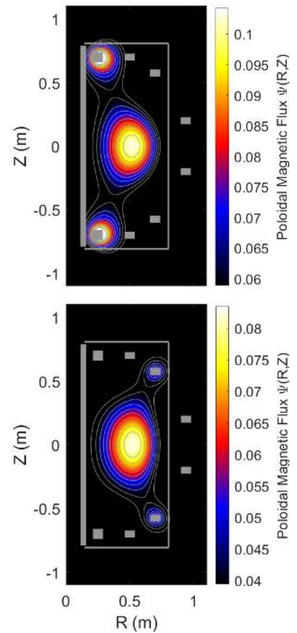
Figure 1. Examples of positive triangularity (upper figure) and negative triangularity (lower figure) plasmas designed for SMART
