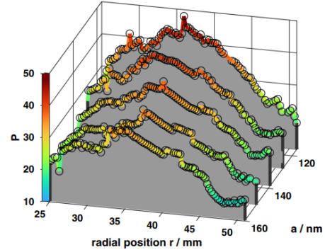
Figure 1: Havnesparameter P for different dust radii (and dust density) along the radial direction. See Ref. [3].
