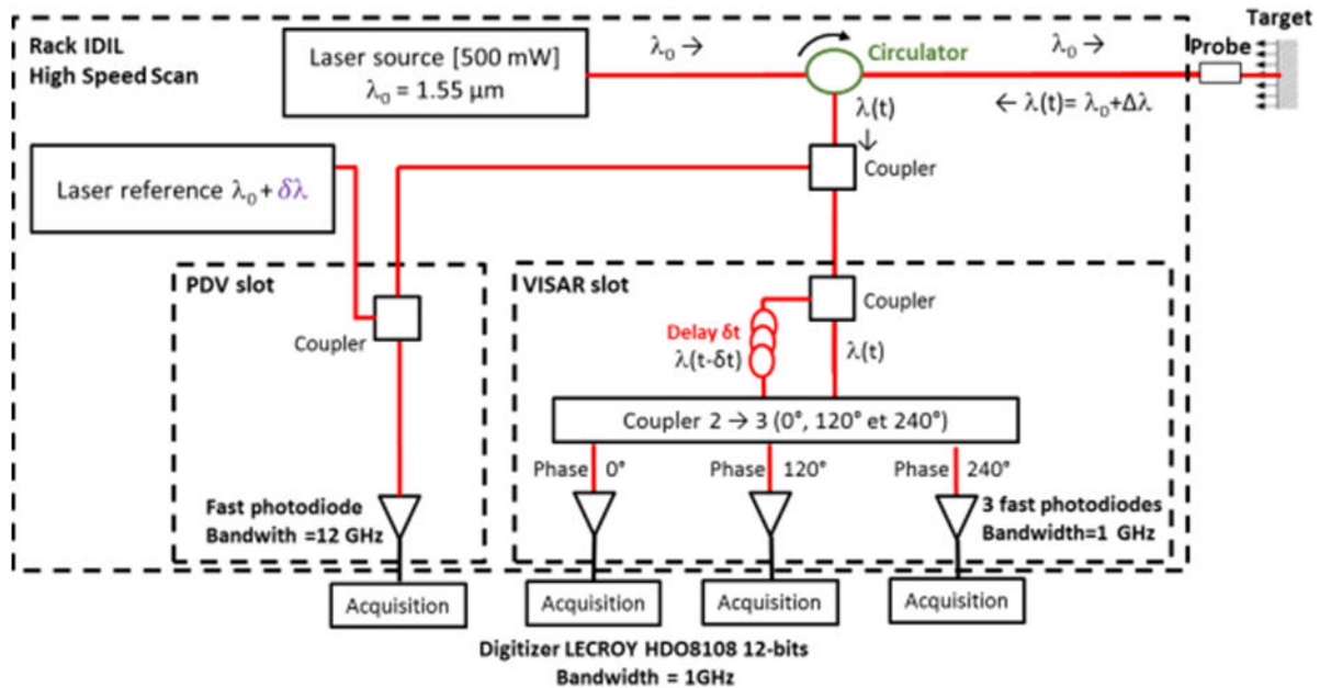
Figure 1: Schematics of our coupled PDV and triature VISAR acquisition system.
