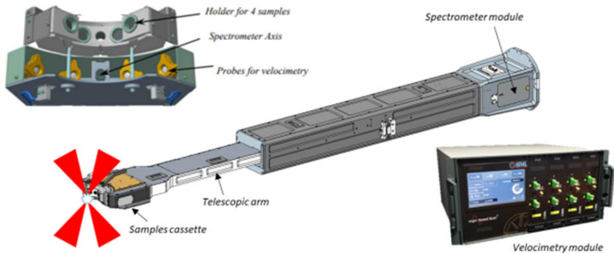
Figure 3: CAD drawings of the LMJ diagnostic dedicated to the study of materials behavior under X-ray irradiation. This device holds four samples in the vicinity of TCC at a distance of 70 or 100 mm. PDV/VISAR channels are connected to the samples; a spectrometer module, made of 4 X-ray diodes with different filters, is used to characterize the X-ray flux which irradiates the samples.
