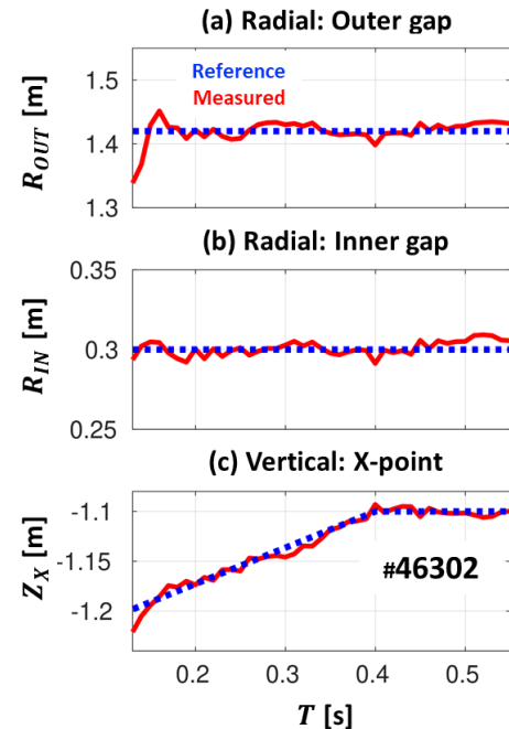
Figure 1. Experimental performance of the shape controller for a MAST-Upgrade Super-X plasma configuration. (a-c) Comparison between the measurement and the reference for R_{IN} , R_{OUT} and Z_X .
