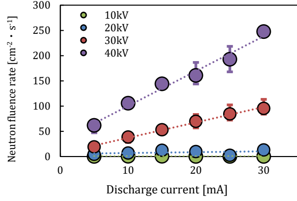
Figure 3: Dependence of neutron fluence rate on discharge current
