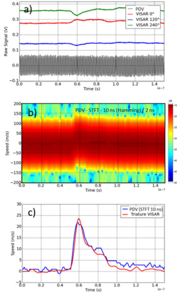
Figure 2: Example of velocity measurements of the rear surface of an Aluminium target irradiated by the BELENOS laser (a) PDV/VISAR raw signals, (b) PDV spectrogram, resulting from an STFT analysis and (c) the derived PDV and VISAR velocities.
