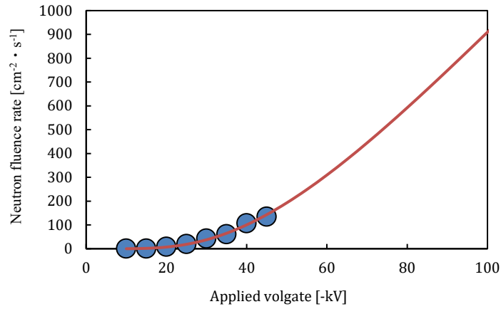
Figure 4: The solid line shows the predicted neutron fluence rate of the discharge current of 10mA when applied voltage is increased to 100kV. The distance from the neutron source is 15 cm.
